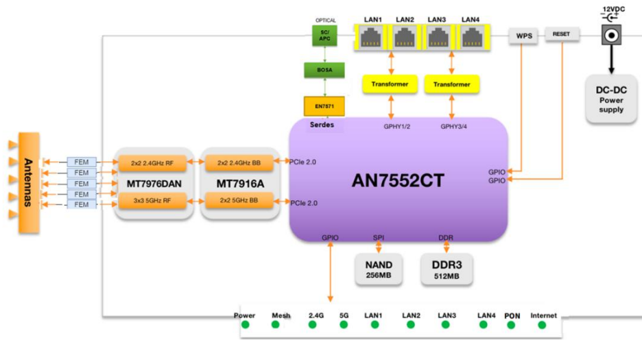
Figure 3: Internet Hub AX3000S Hardware Block Diagram
